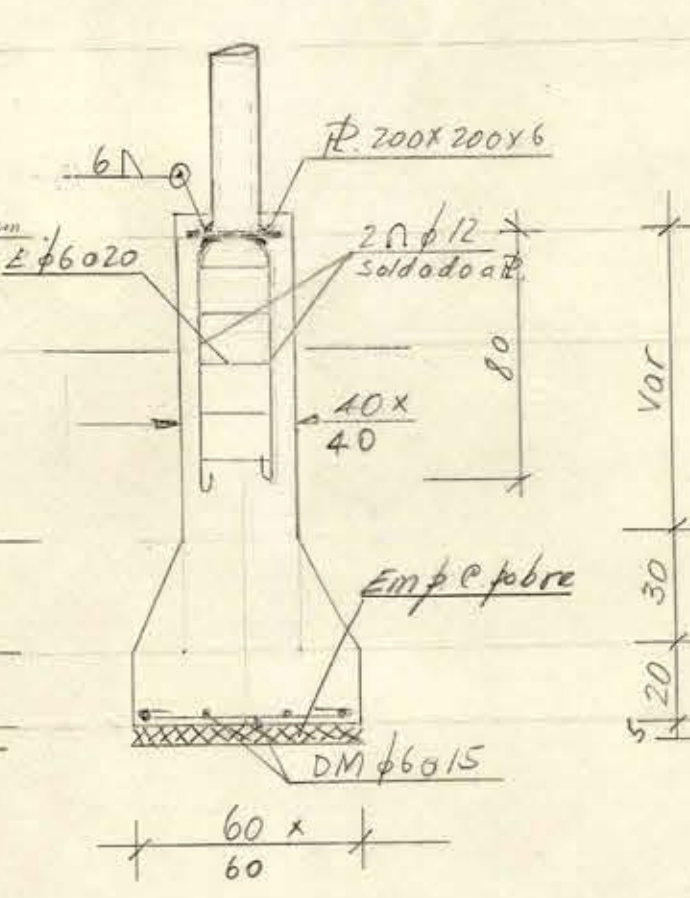
Fund. P10.
