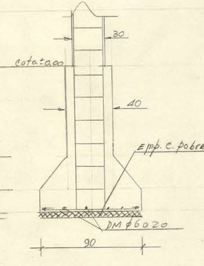
Fund. P11
