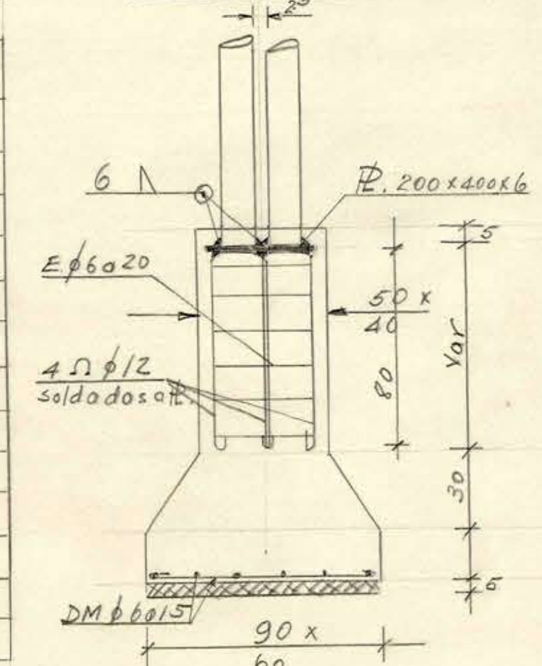
Fund. P10+P11
