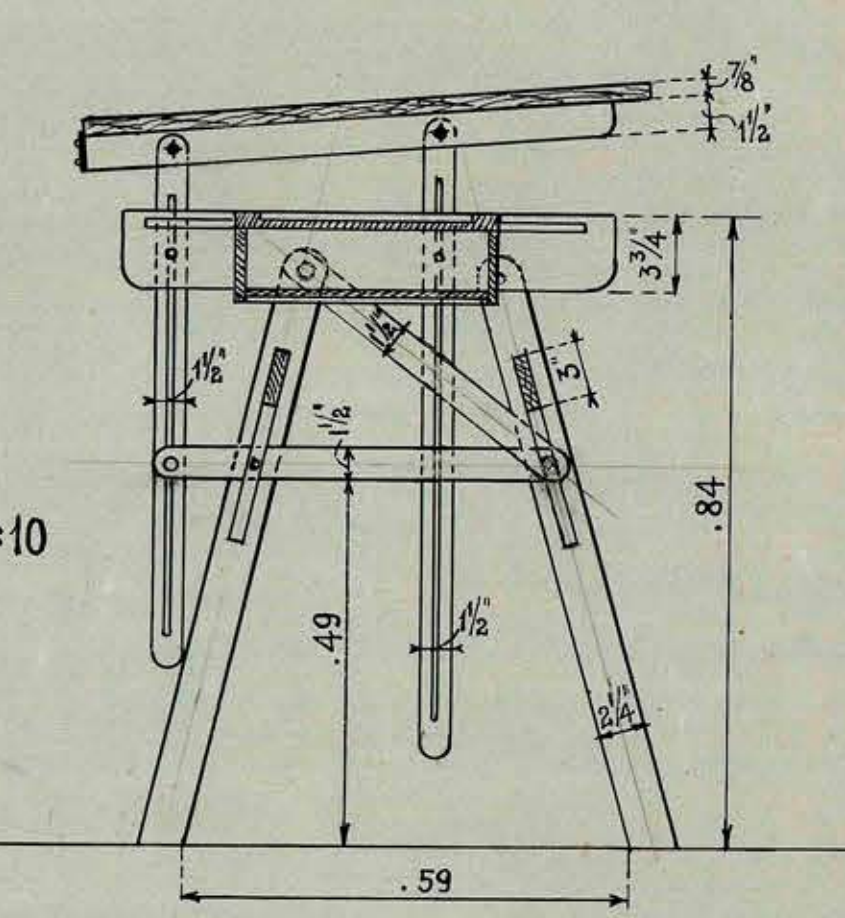
ELEVACION "D"
