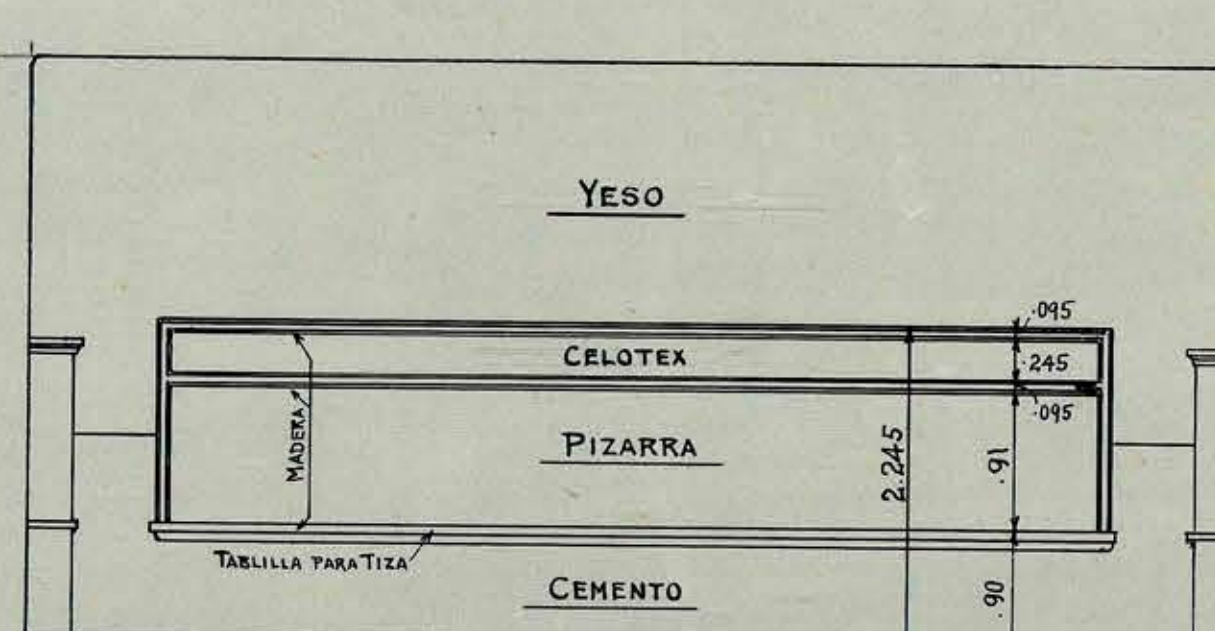
ELEVACION "D"
