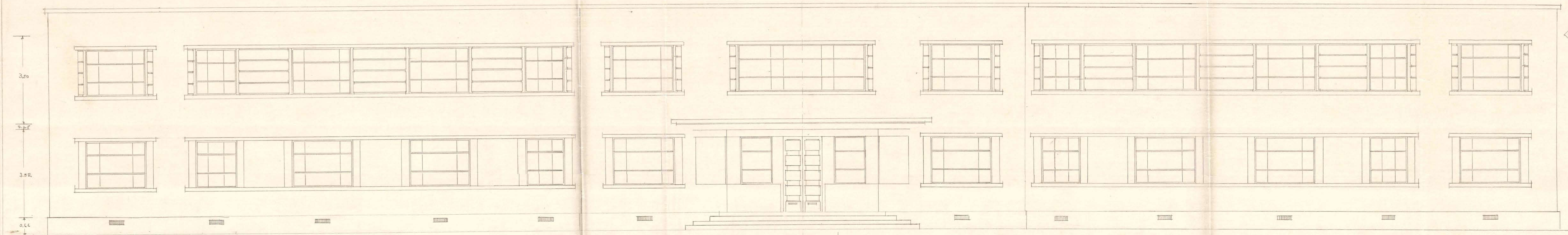
FACHADA PRINCIPAL
