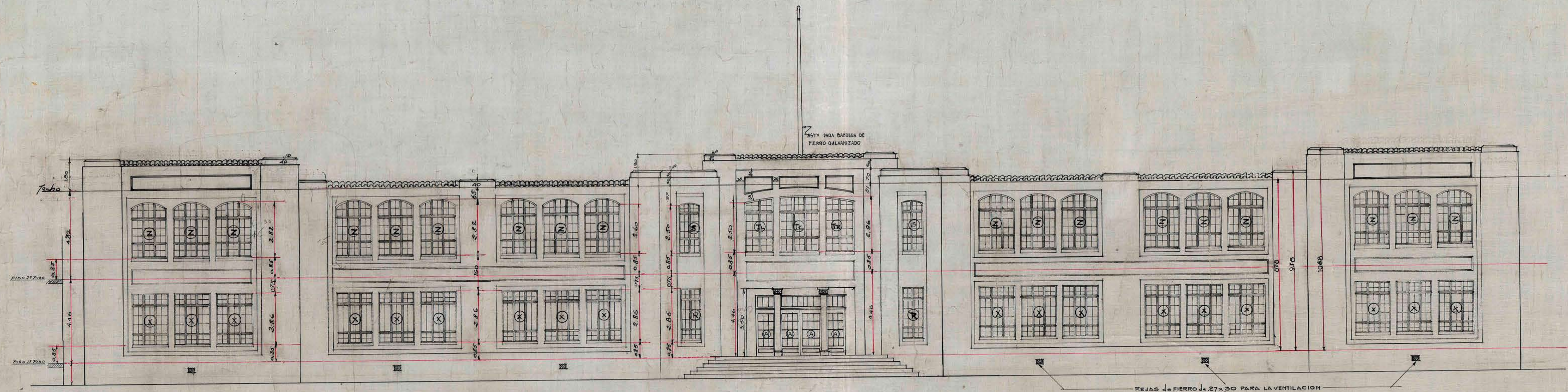
FACHADA PRINCIPAL
