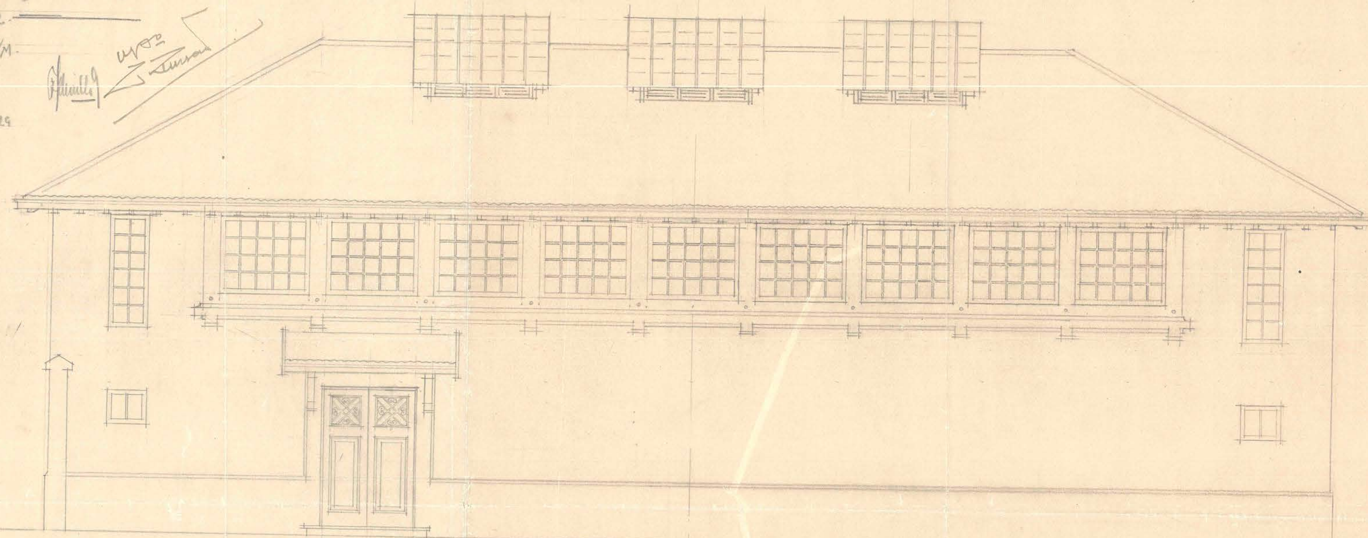
FACHADA PRINCIPAL
