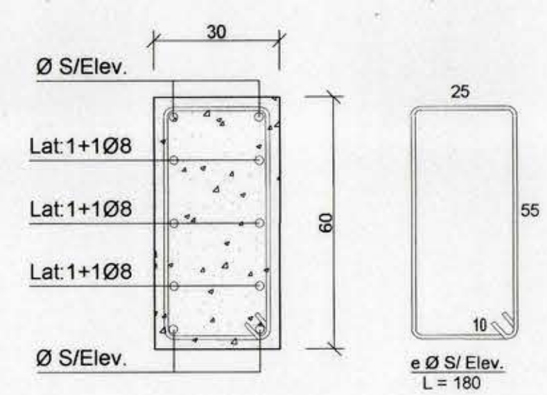
SECCION V. 30/60 ESCALA 1:12.5
