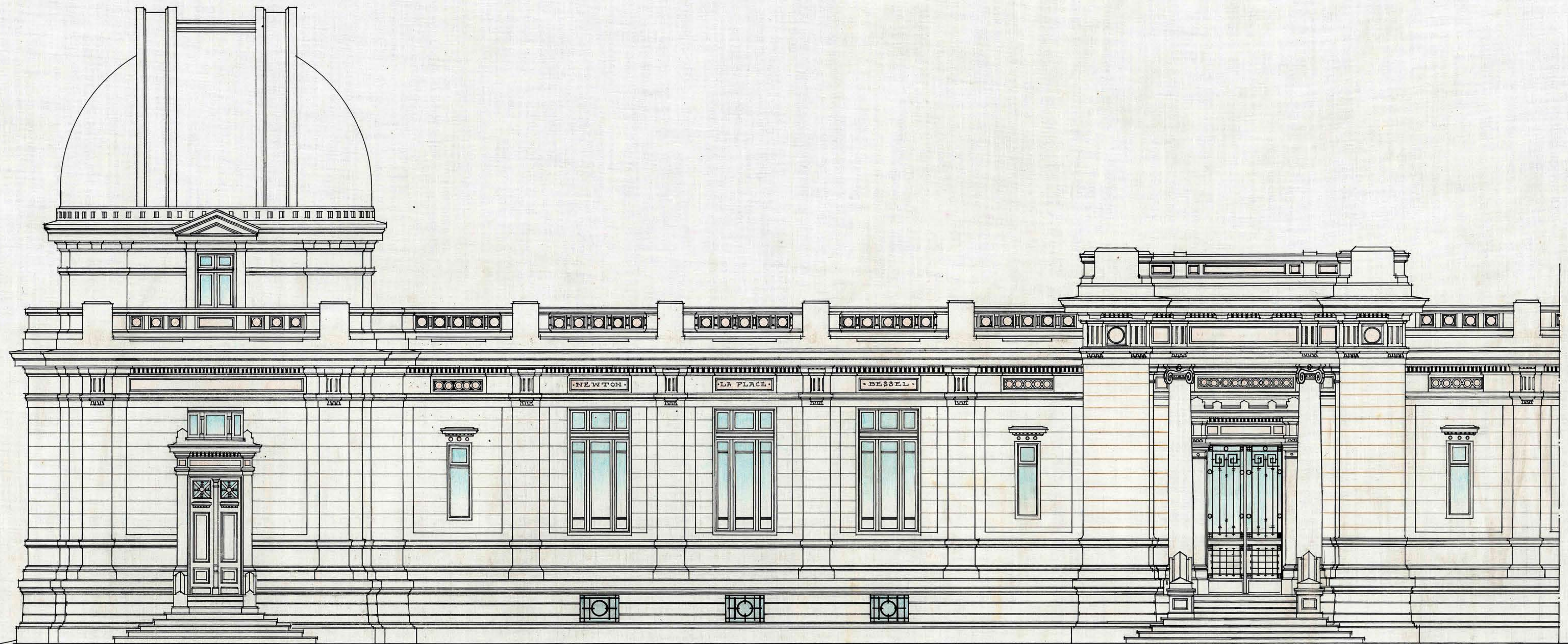
← ELEVACION PRINCIPAL →
