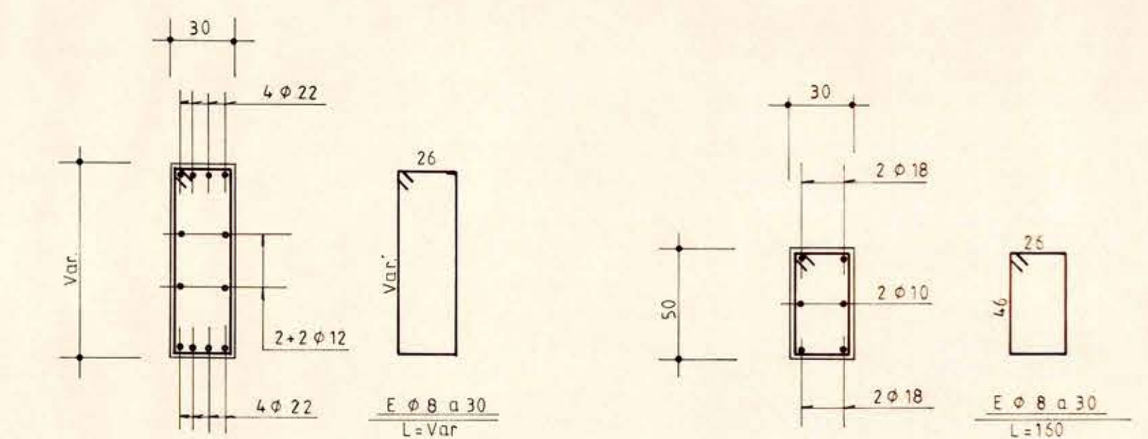
PILAR P1 30/Var. SIMILAR P6 30/Var
