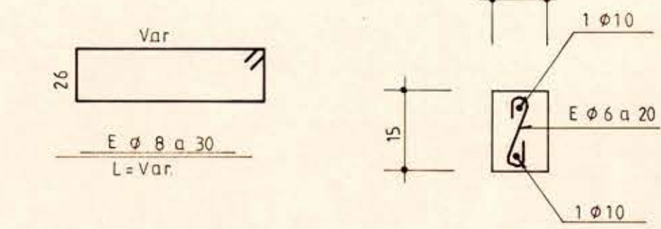
PILAR P5 10/15 SIMILAR CADENETA 10/15
