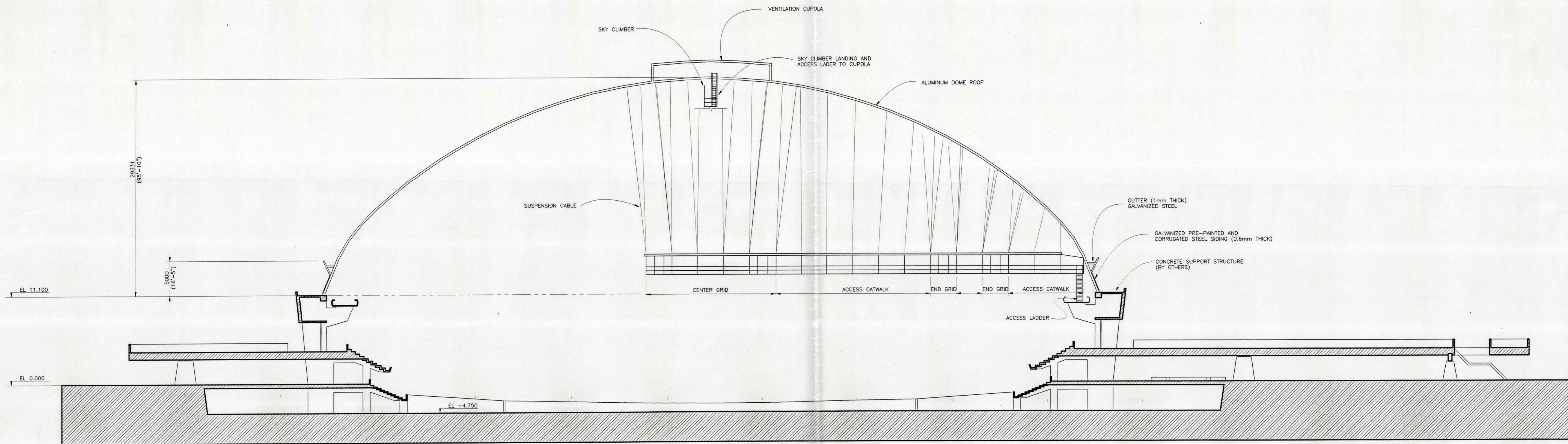
BUILDING SECTION NORTH
