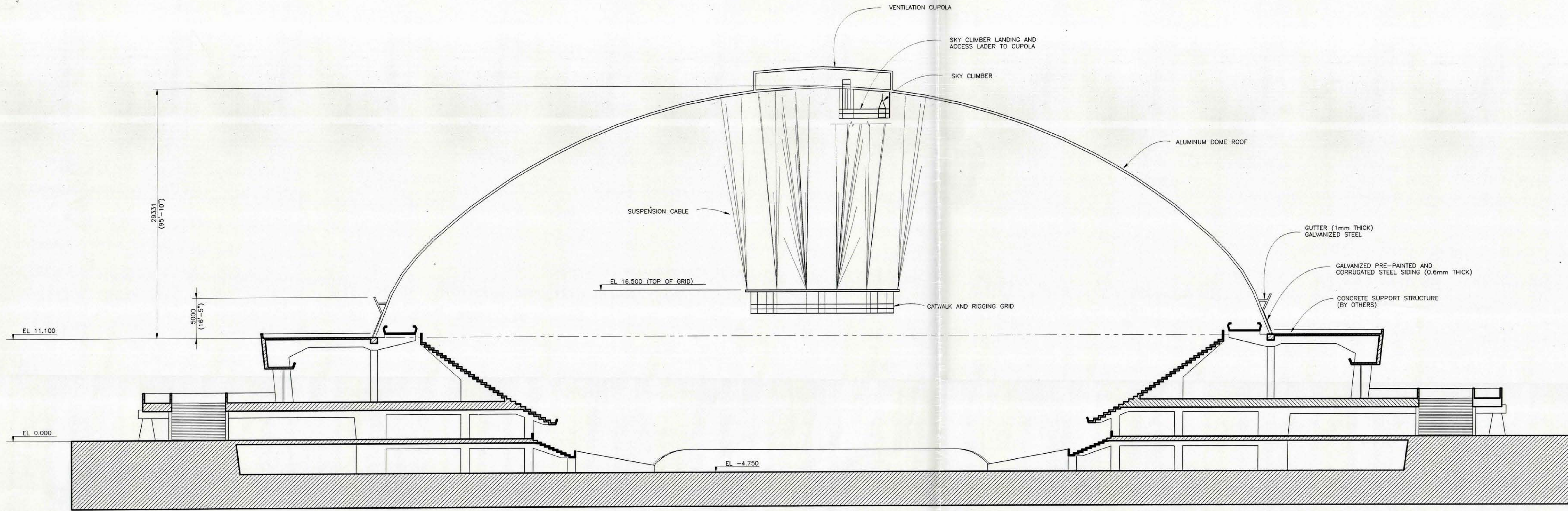
BUILDING SECTION EAST
