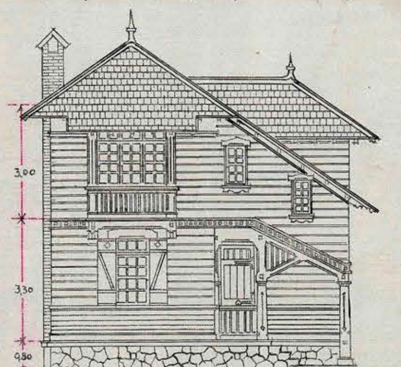
FACHADA PRINCIPAL
