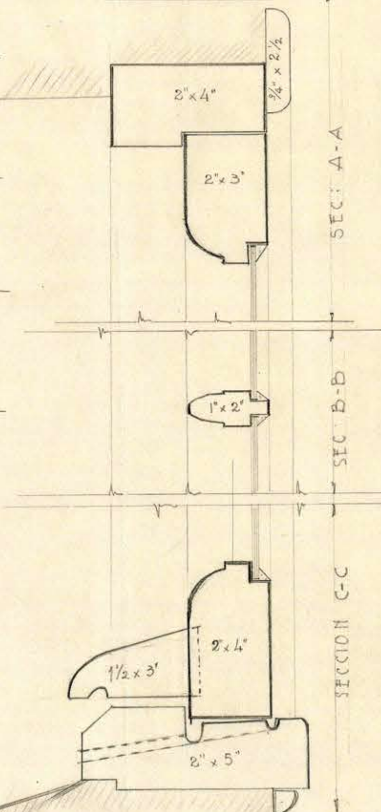
CORTE VERTICAL
