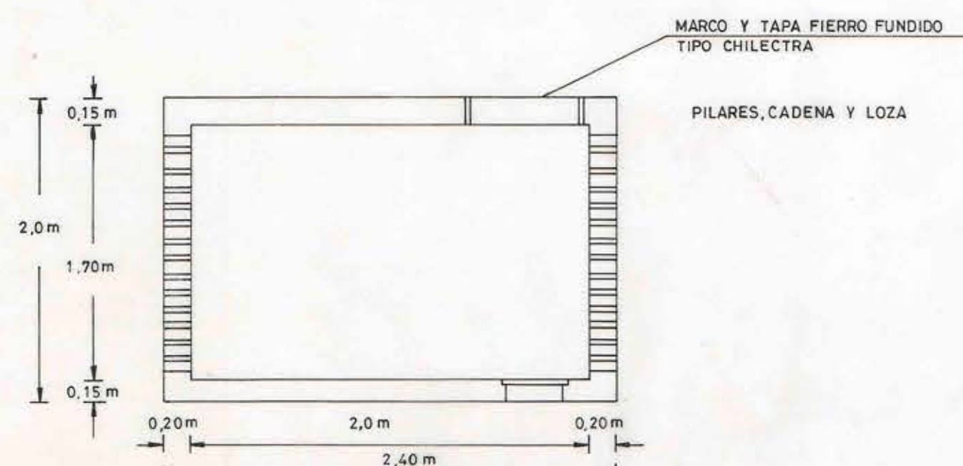
DETALLE CAMARA 2,0 x 2,0 x 1,7mts
