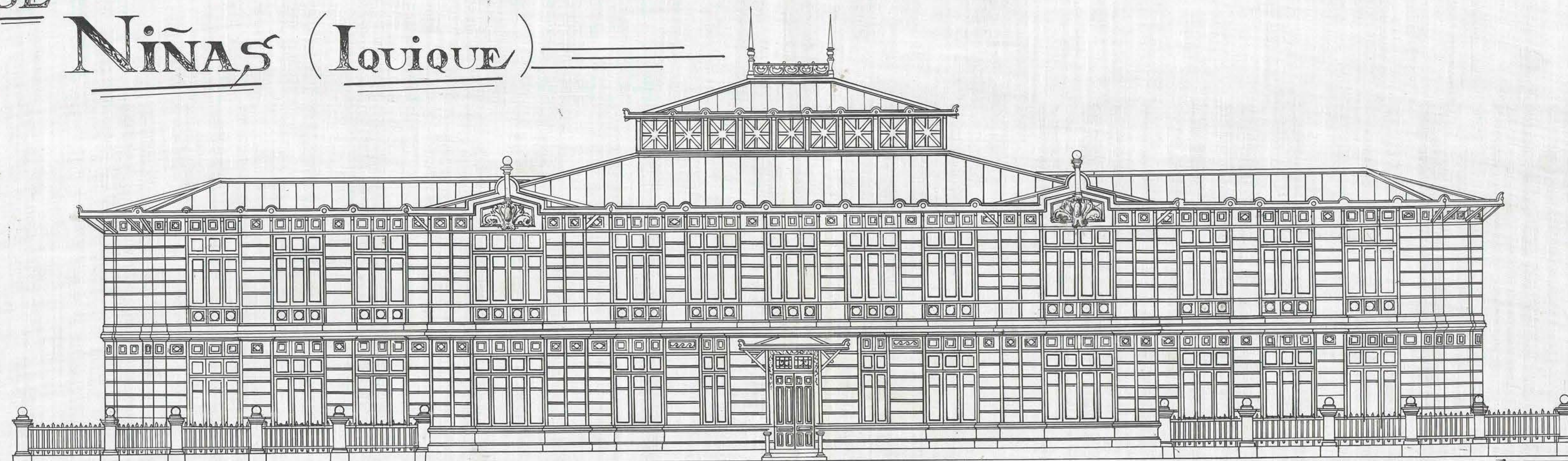
FACHADA PRINCIPAL
