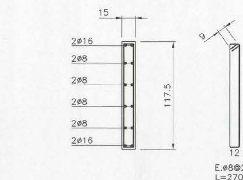
DETALLE V.15/117.5 ESCALA 1:25
