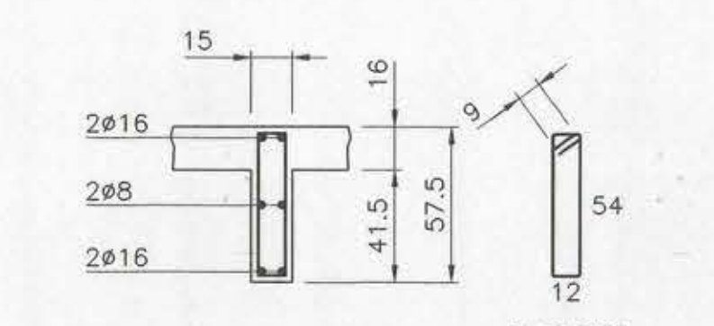
DETALLE V.15/57.5 ESCALA 1:25
