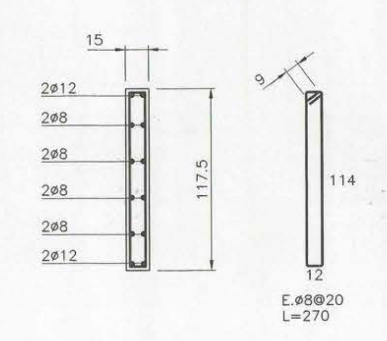
DETALLE V.15/117.5 ESCALA 1:25
