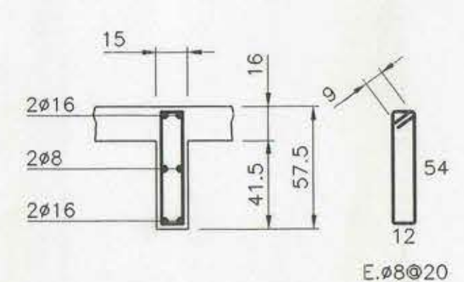
DETALLE V.15/57.5 ESCALA 1:25
