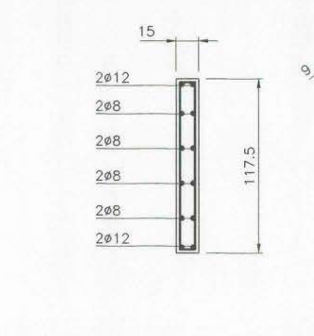
DETALLE V.15/117.5 ESCALA 1:25
