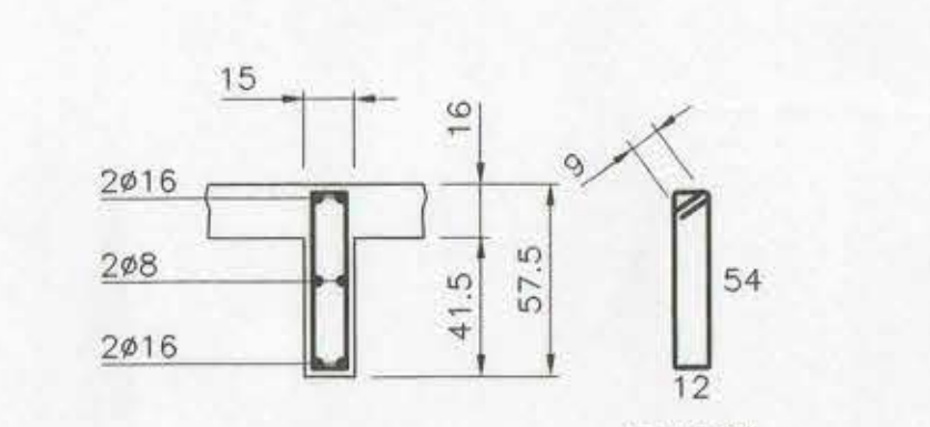
DETALLE V.15/57.5 ESCALA 1:25
