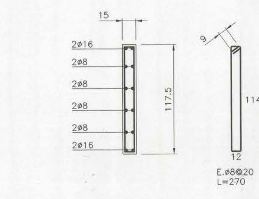
DETALLE V.15/117.5 ESCALA 1:25
