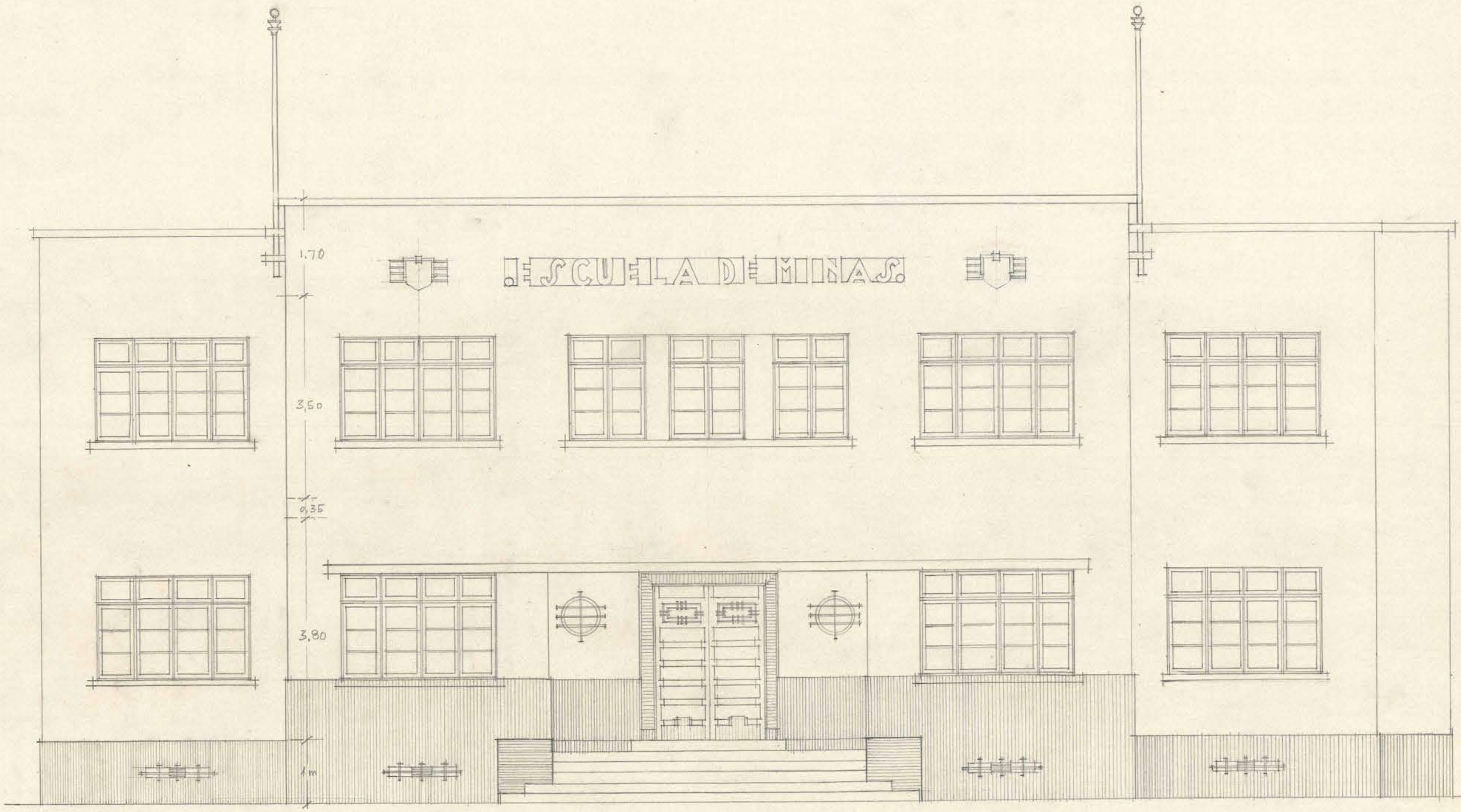
FACHADA PRINCIPAL
