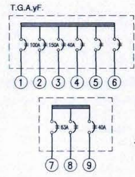
DIAGRAMA UNILINEAL
