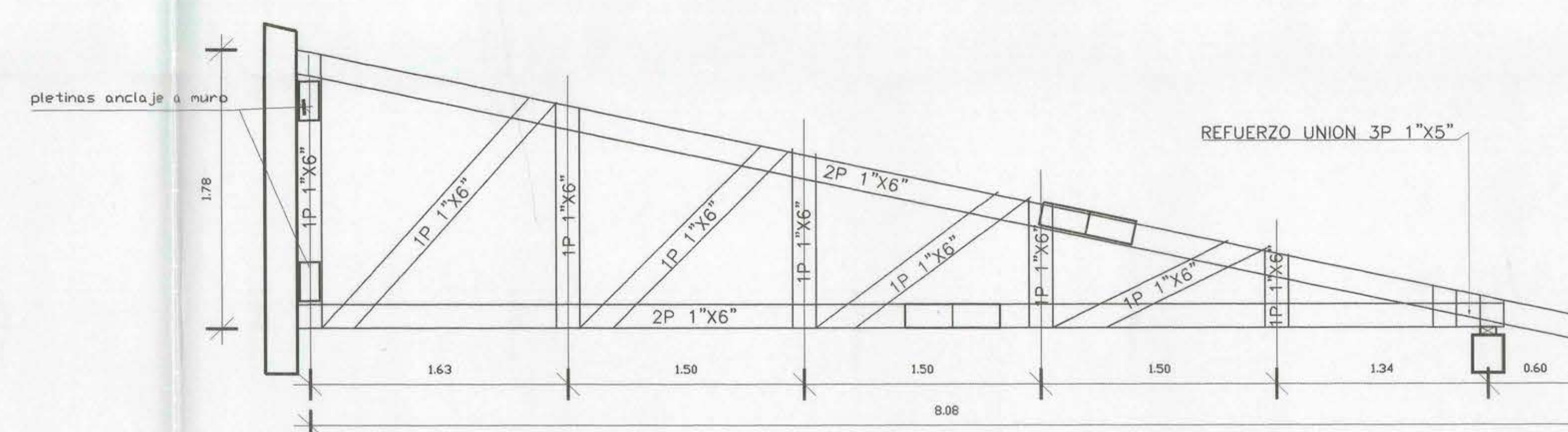
CERCHA 1C
