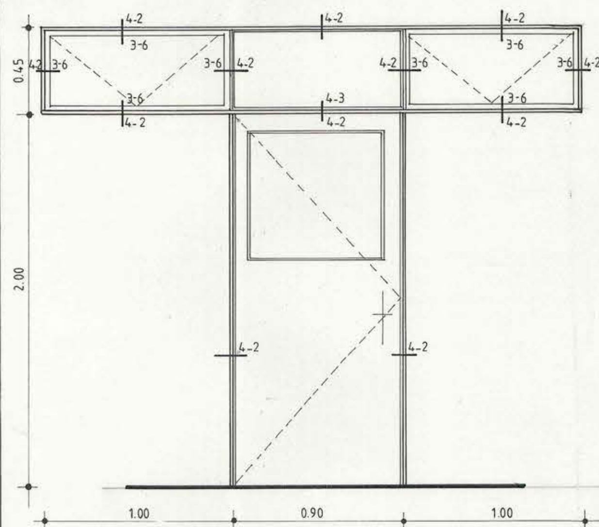
PUERTA P1 (SON 2) ESC. 1:20
