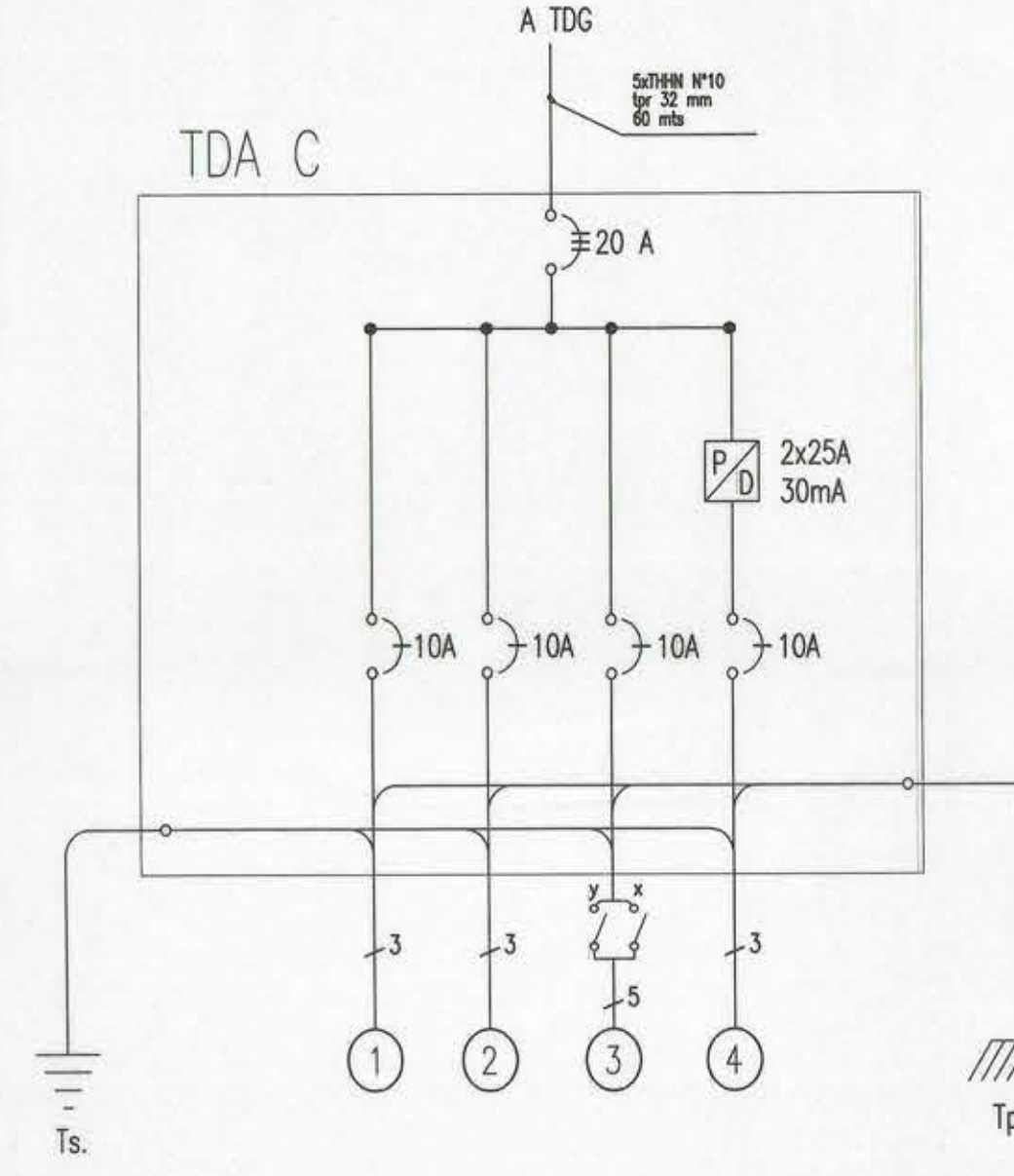
DIAGRAMA UNILINEAL TDA C
