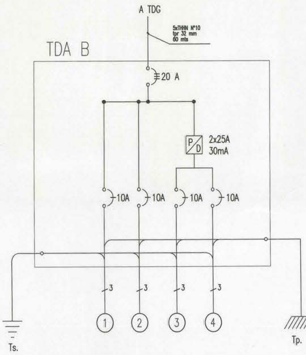
DIAGRAMA UNILINEAL TDA B
