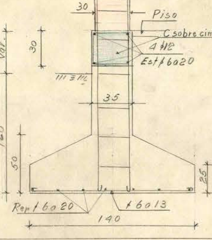
Fund. Pilar 24
